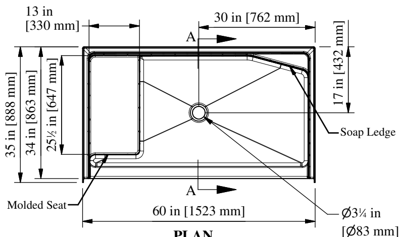
60" [1523mm] Shower w/ 3" [74mm] Threshold & Molded Seat and Soap Ledge
